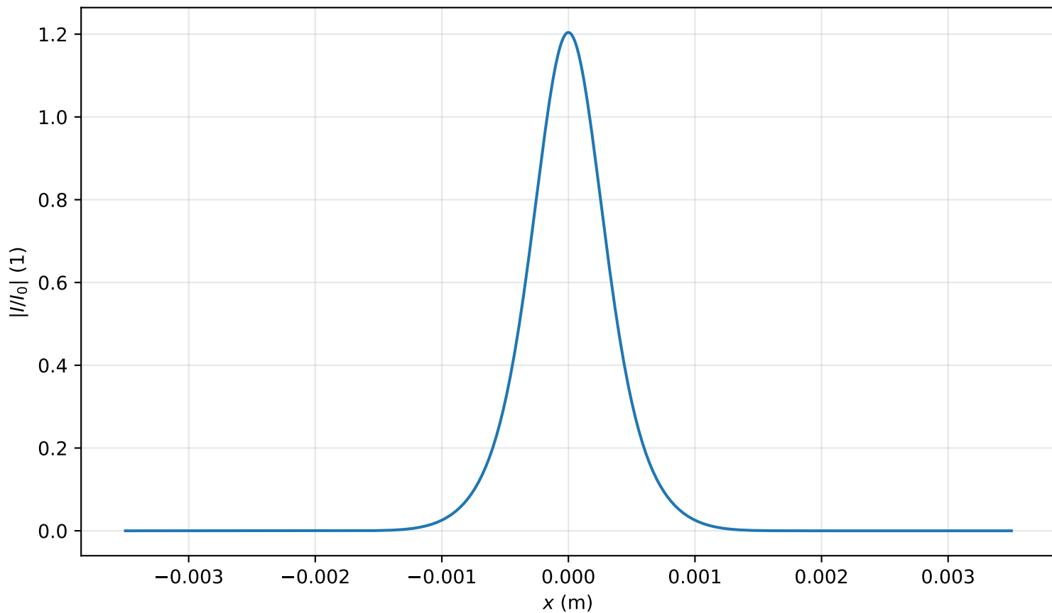
Intensity profile I(x, y = 0, z = 1.035m)/I_0 , P_{in}=0.7P_{cr} , artificial time
